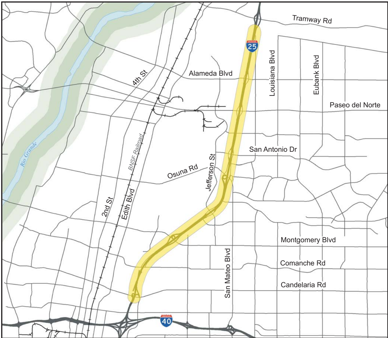
Project Location Map North I-25 Freeway Operations Study TPA-TPU-025-4(122)228, CN D3018 Albuquerque, Bernalillo County, New Mexico
